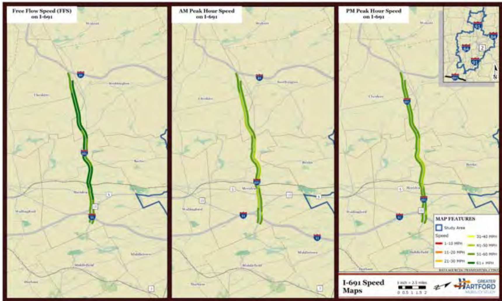
Figure 2-20: I-691 Speed Maps
