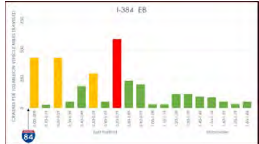
Figure 3-20: I-384 Eastbound Crash Rates
